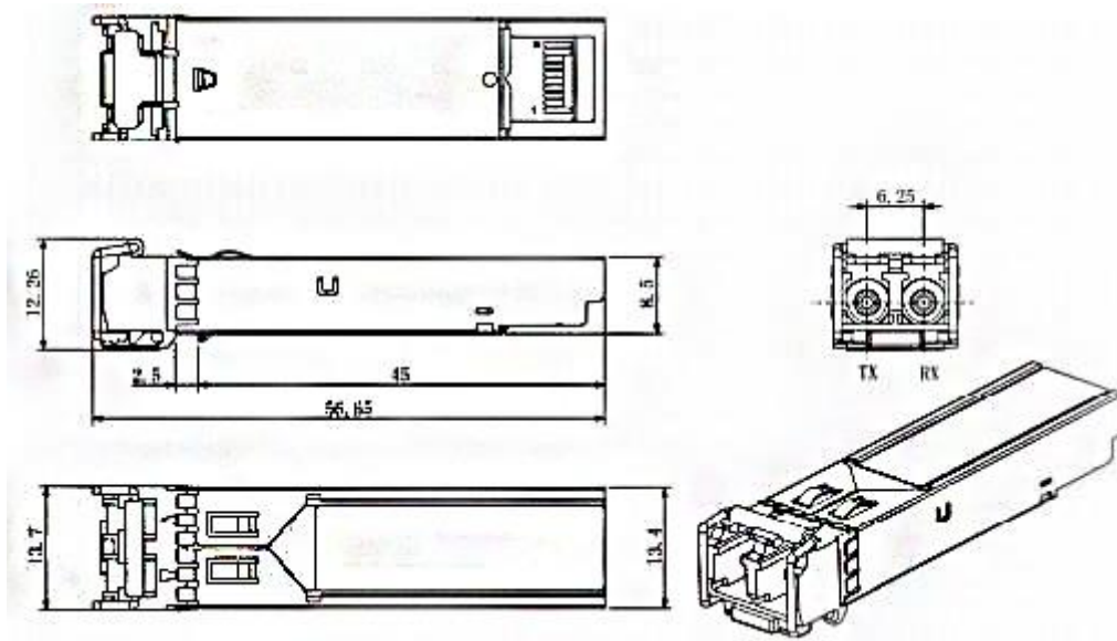
Mechanical Drawing
